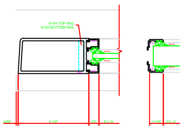
300 STILE 3/4 DIA FOR OFFSET PIVOT/BUTT HINGE
