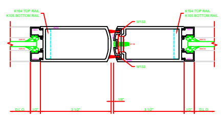
400 MEETING STILE 3/4 DIA
