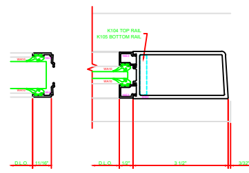
305 STILE 3/4 DIA FOR OFFSET PIVOT/BUTT HINGE
